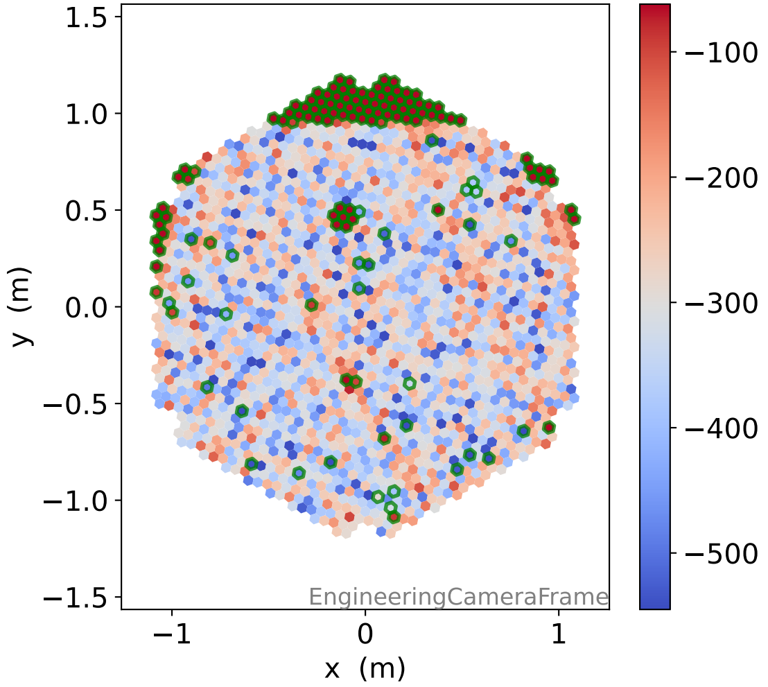
HG photon-electrons
