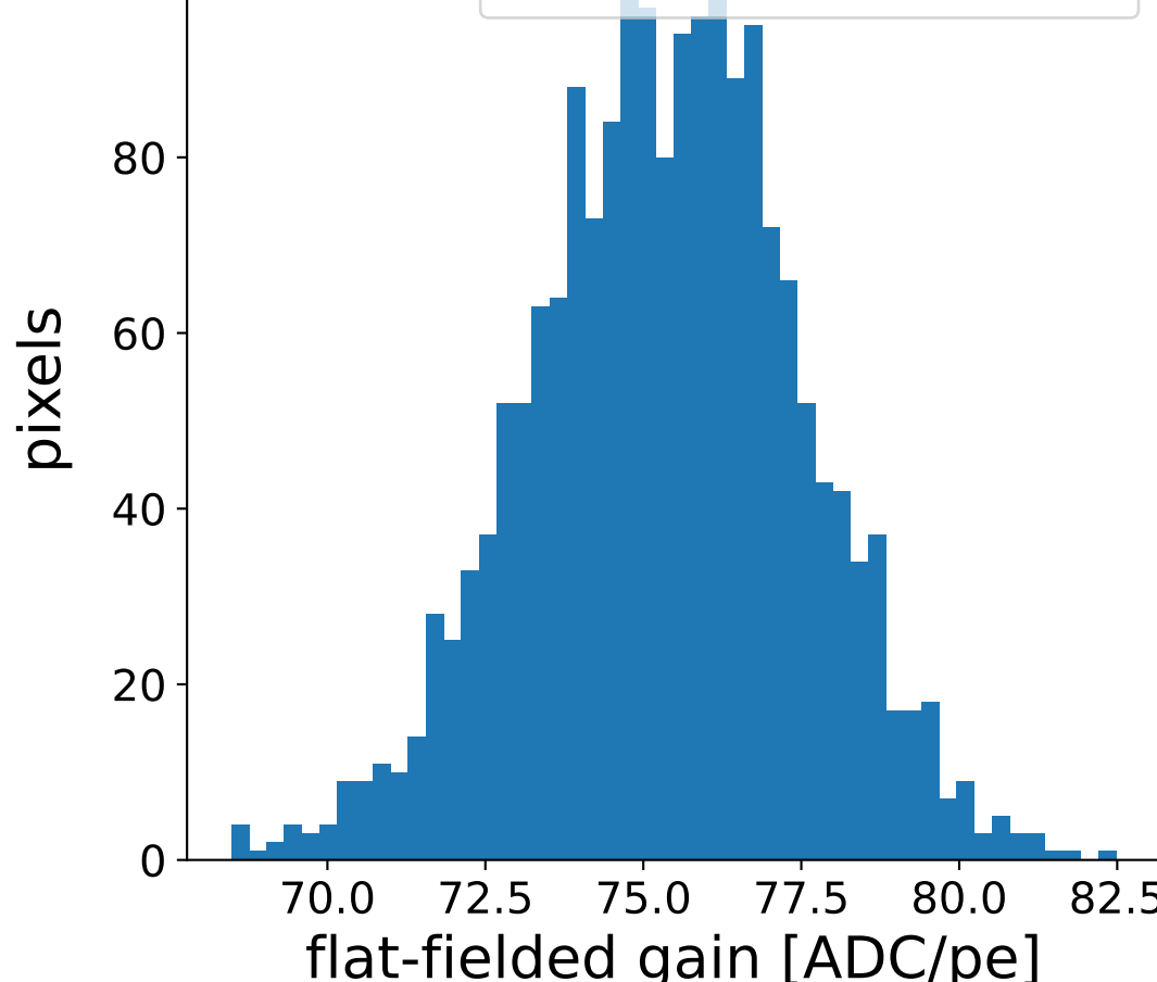
Median 75.40, std 2.14
