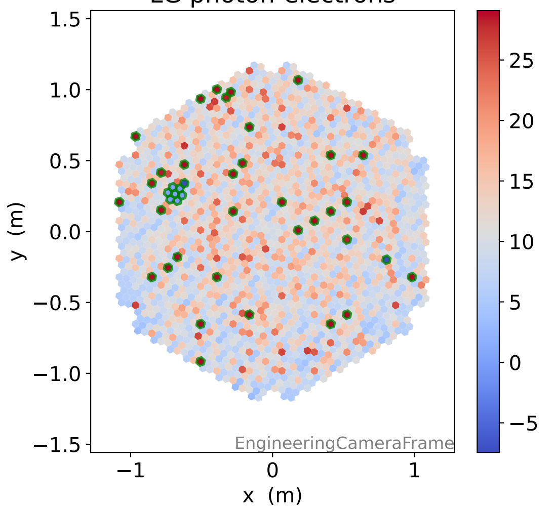
LG photon-electrons
