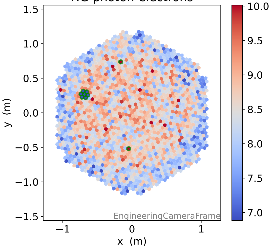
HG photon-electrons
