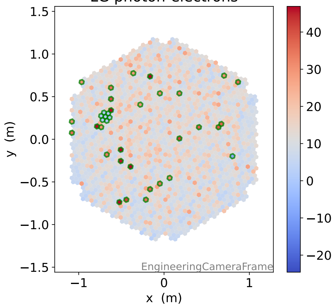
LG photon-electrons
