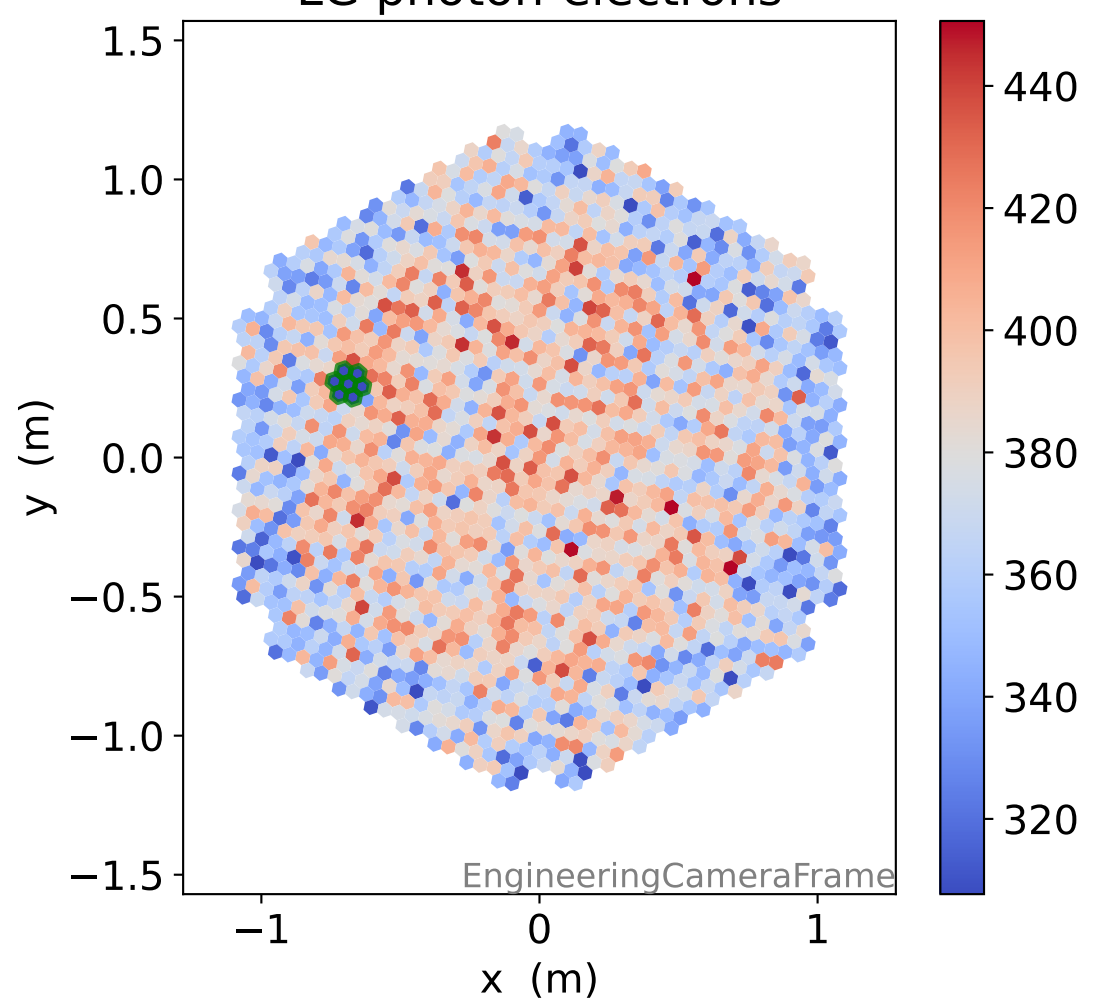
LG photon-electrons
