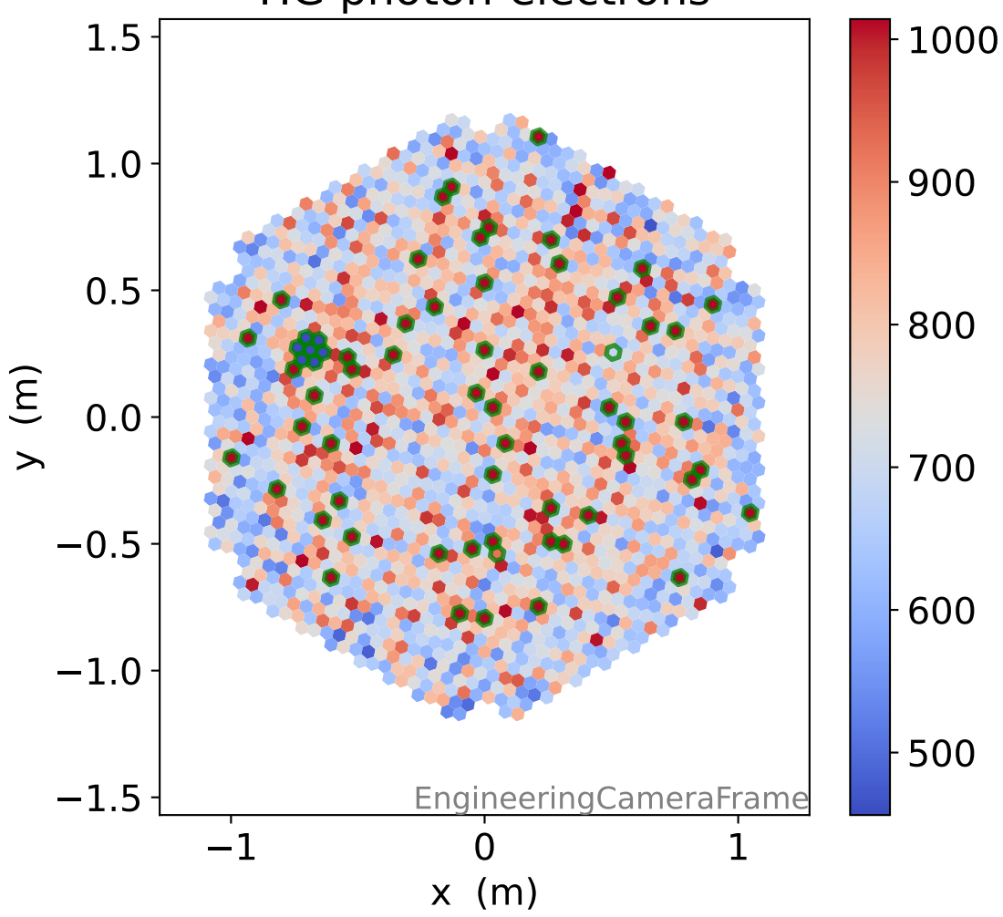
HG photon-electrons
