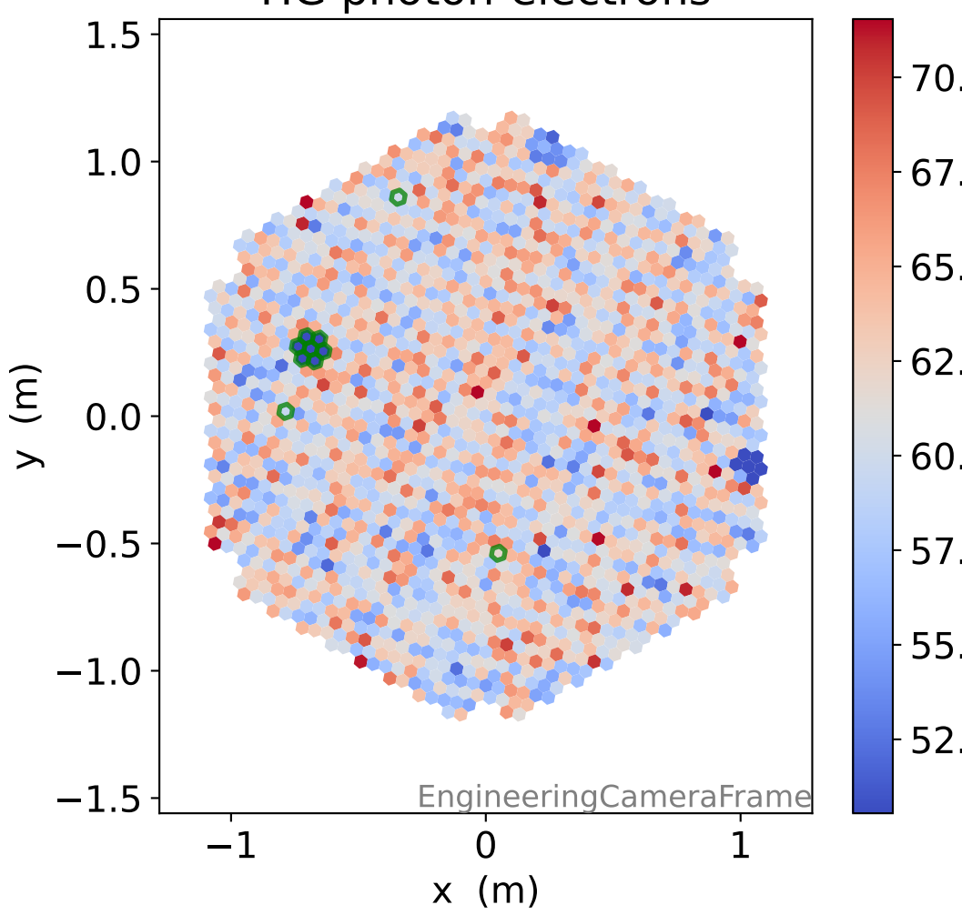
HG photon-electrons
