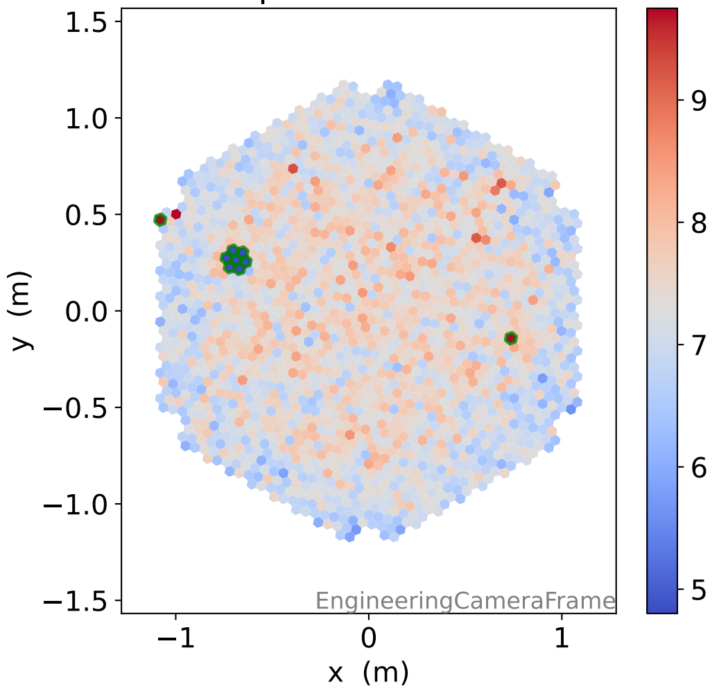
HG photon-electrons
