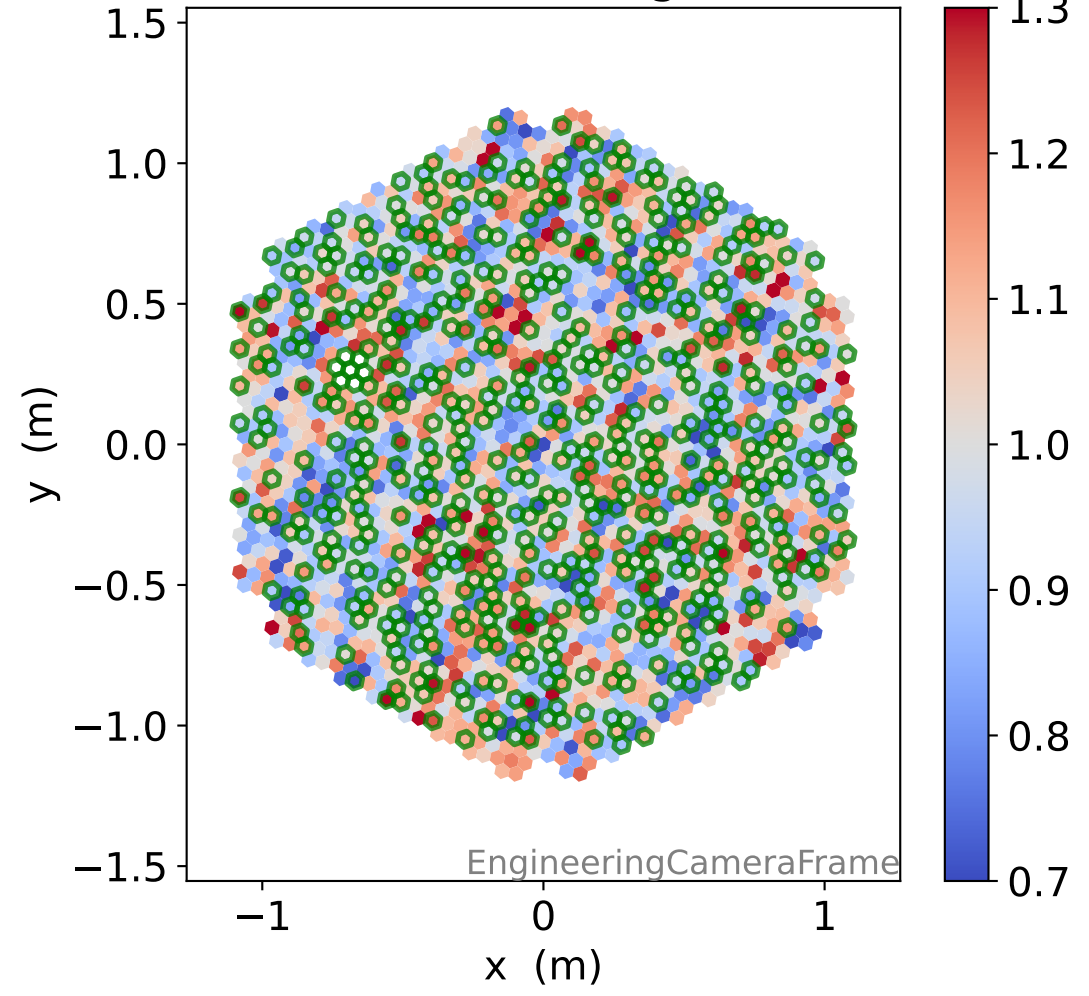
LG photon-electrons
