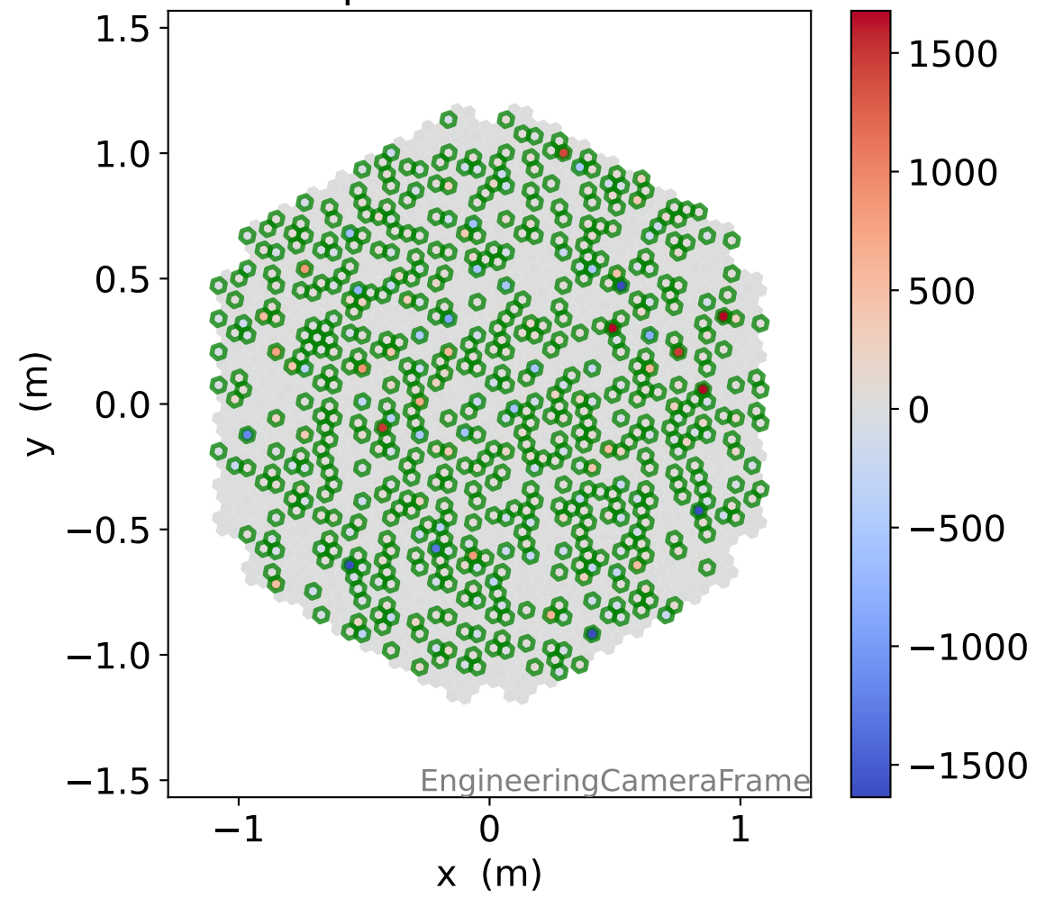
LG photon-electrons
