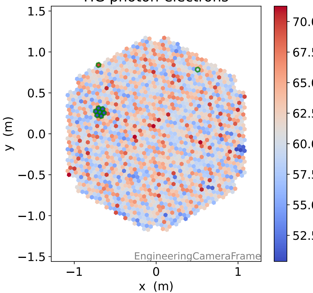
HG photon-electrons
