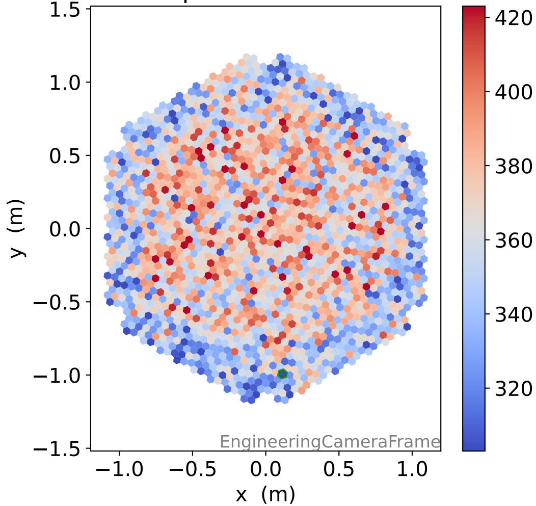
LG photon-electrons
