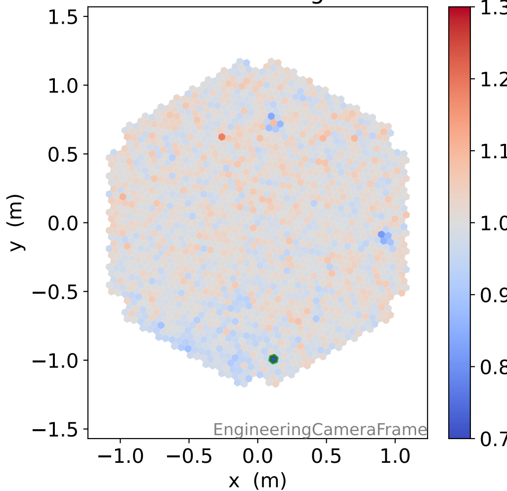
LG photon-electrons
