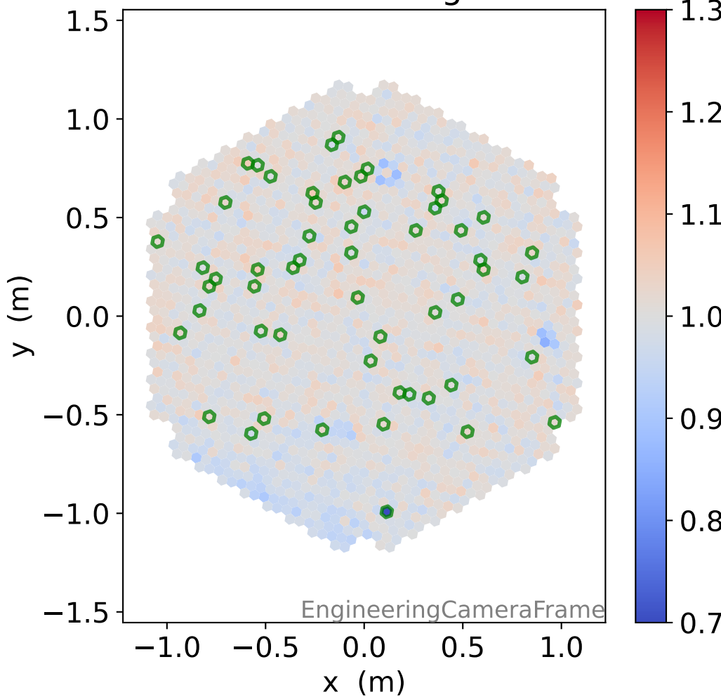
HG photon-electrons
