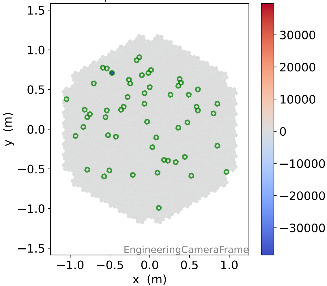
HG photon-electrons
