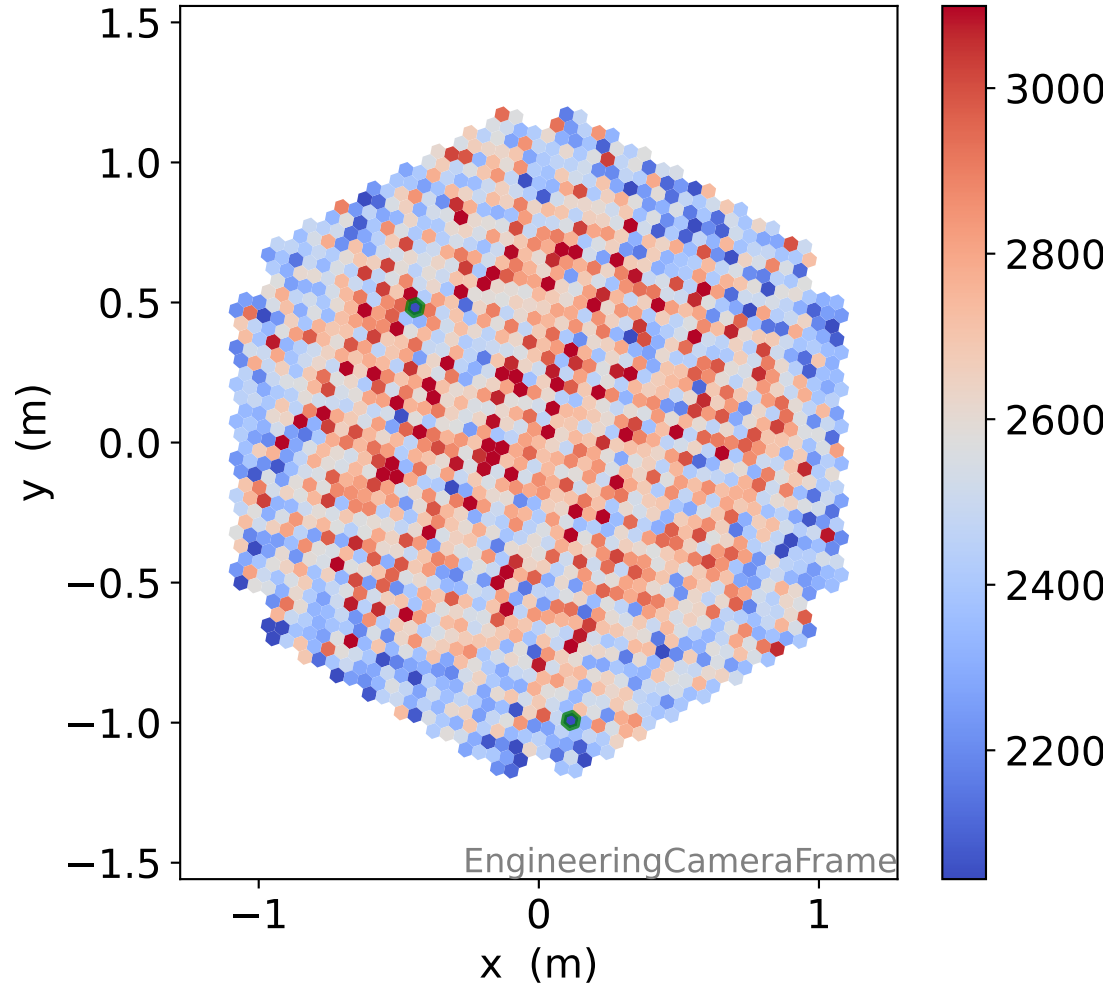
LG photon-electrons
