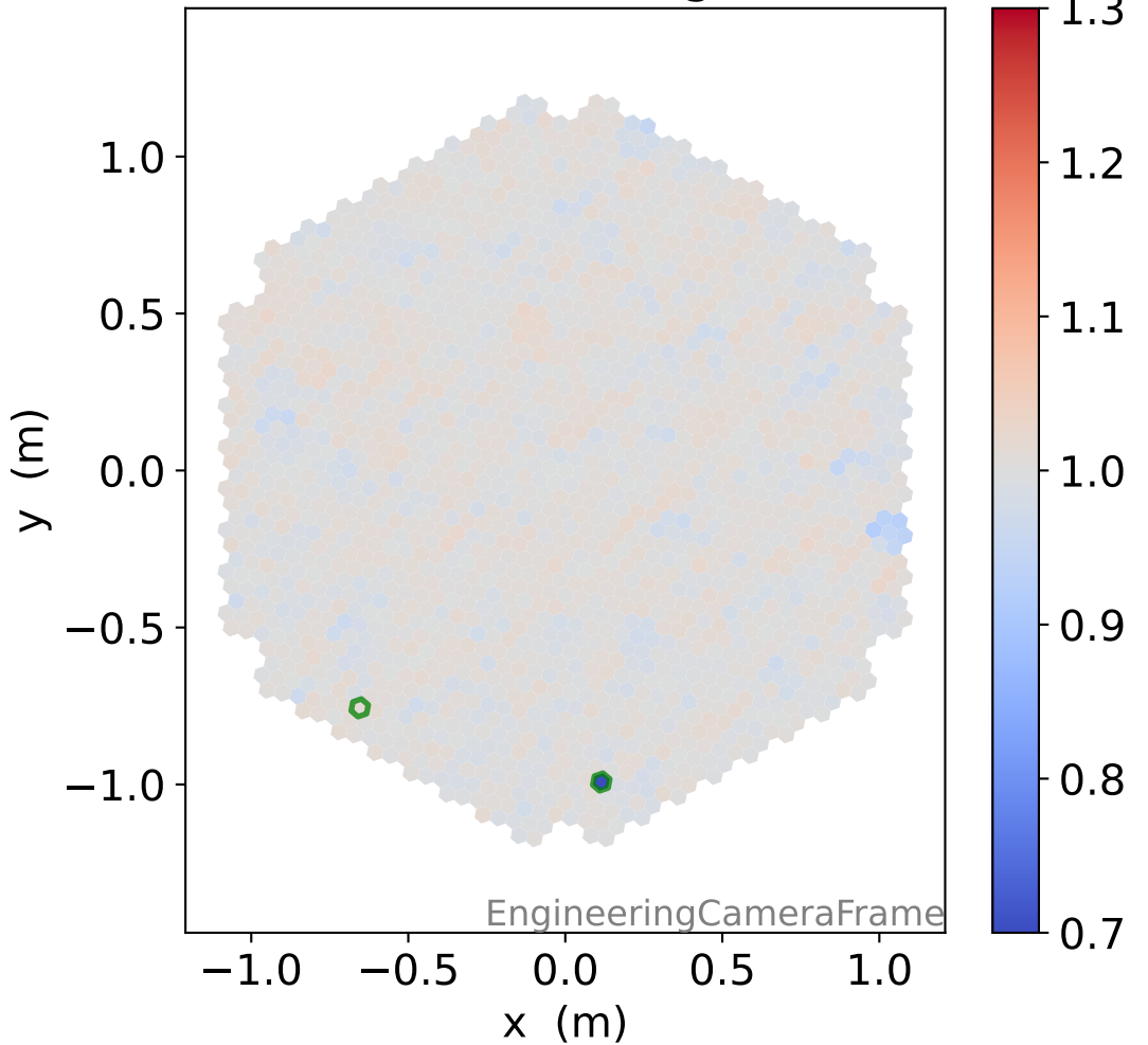
HG photon-electrons
