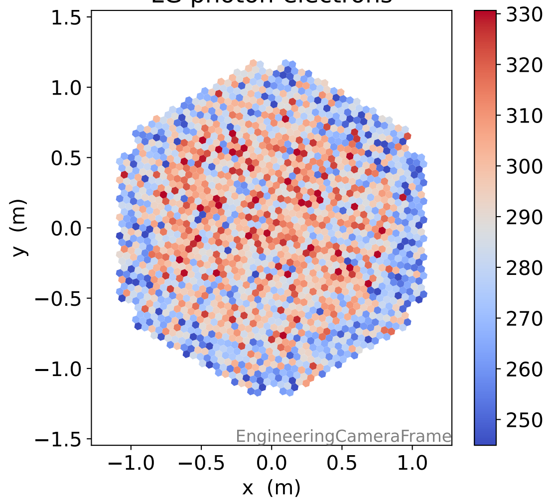
LG photon-electrons
