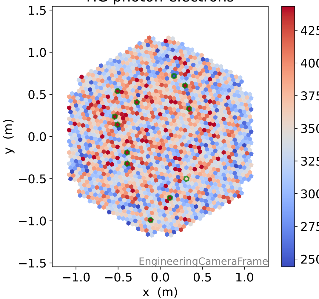
HG photon-electrons
