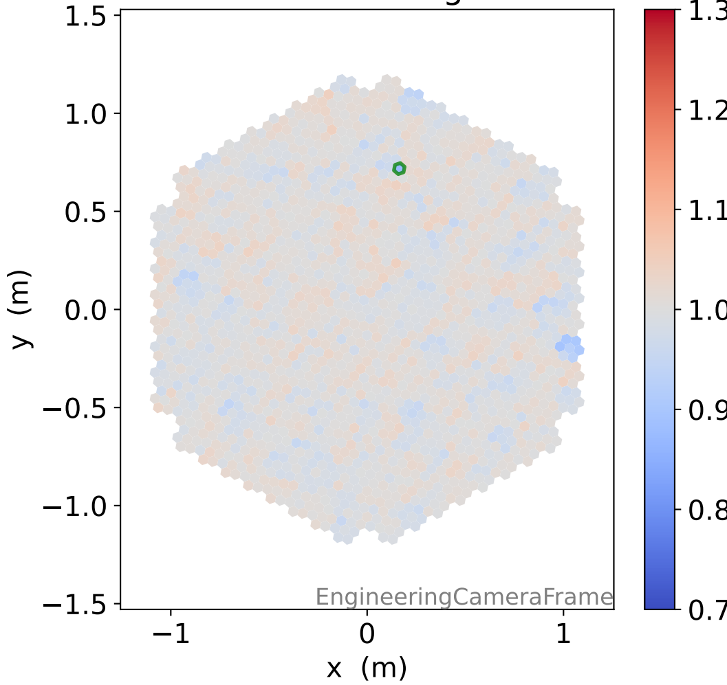
HG photon-electrons
