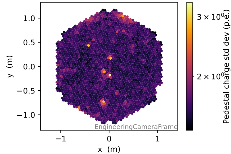
Pedestal charge std dev (p.e.)
