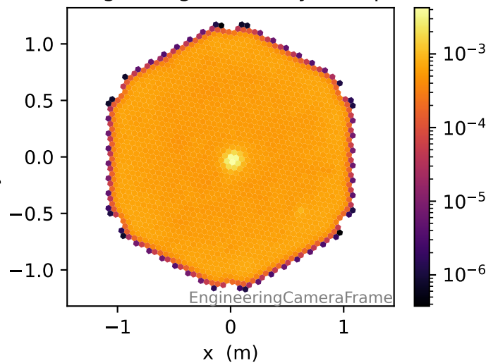
Image c.o.g., intensity > 200pe
