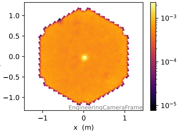
Image c.o.g., intensity > 200pe
