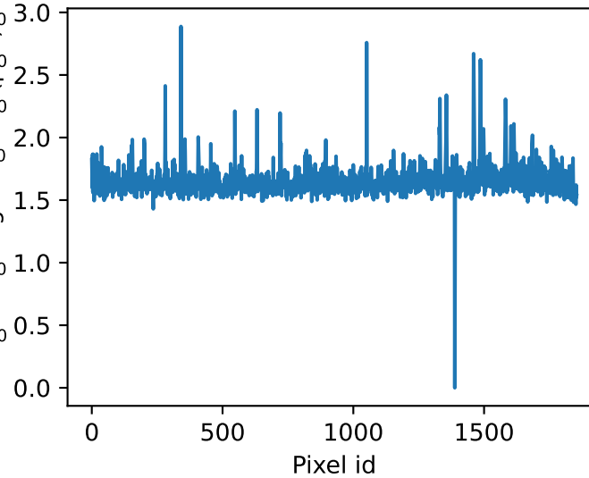
Pedestal charge std dev (p.e.)
