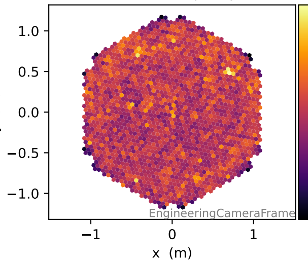
Fraction of >300 p.e. pulses
