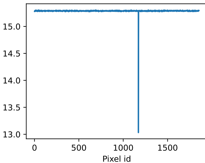
Flat-field mean time (ns)
