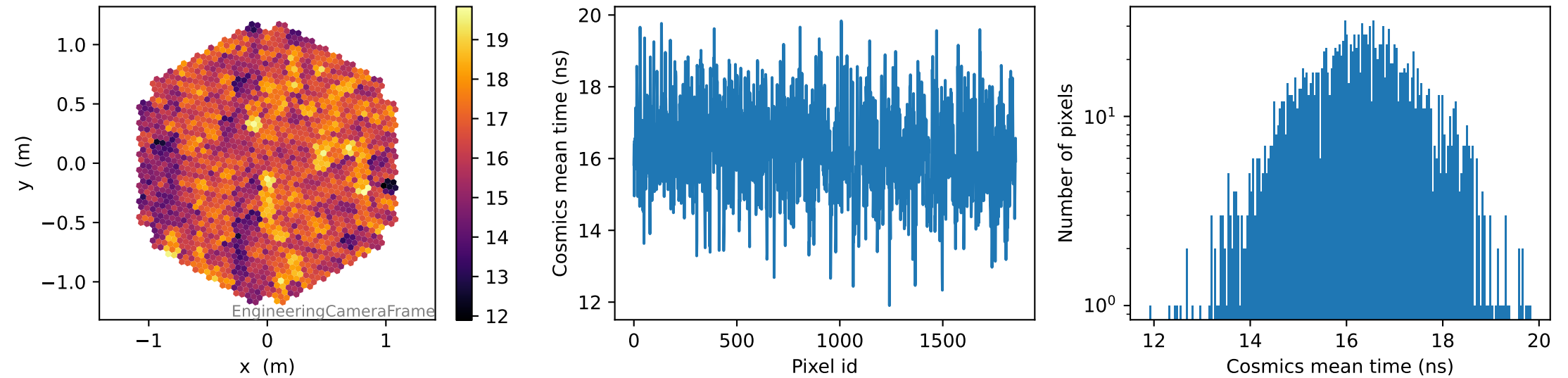
Cosmics mean time (ns)
