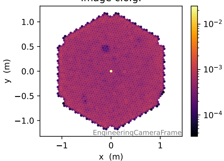
Image c.o.g., intensity > 200pe
