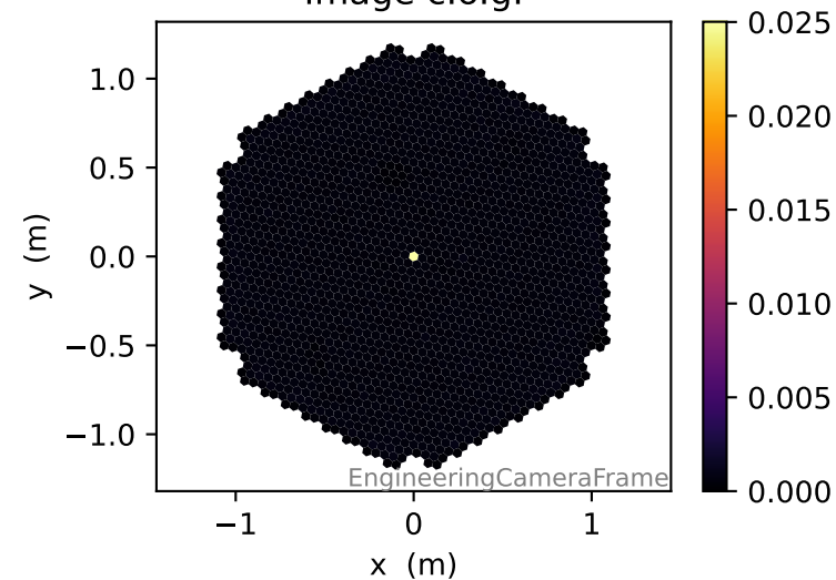
Image c.o.g., intensity > 200pe
